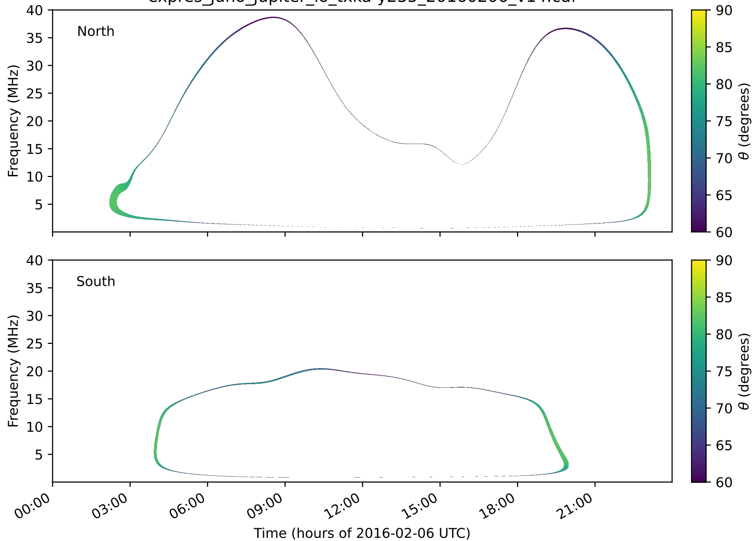
expres_juno_jupiter_io_txka-y235_20160206_v14.cdf
