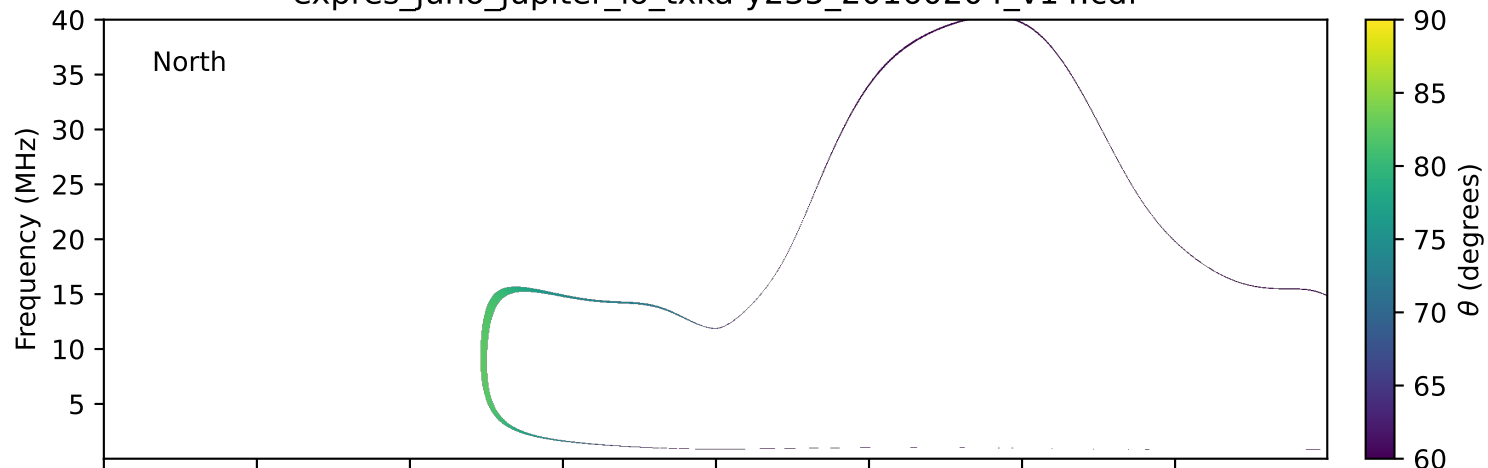
expres_juno_jupiter_io_txka-y235_20160204_v14.cdf
