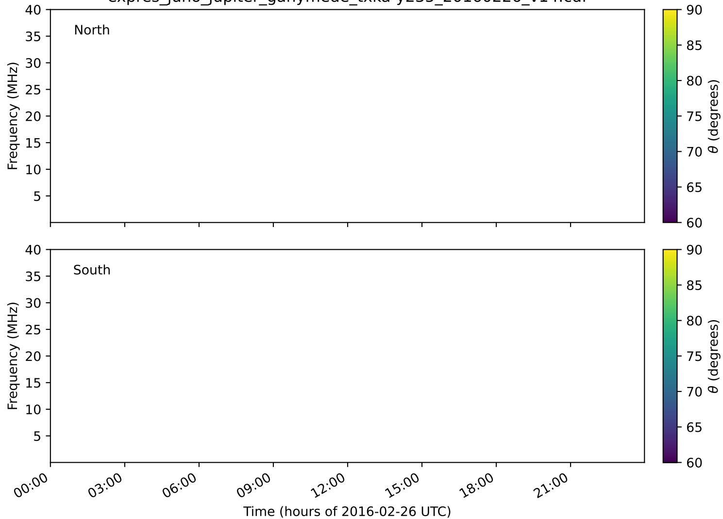
expres_juno_jupiter_ganymede_txka-y235_20160226_v14.cdf
