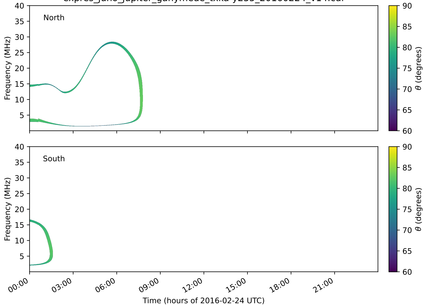
expres_juno_jupiter_ganymede_txka-y235_20160224_v14.cdf
