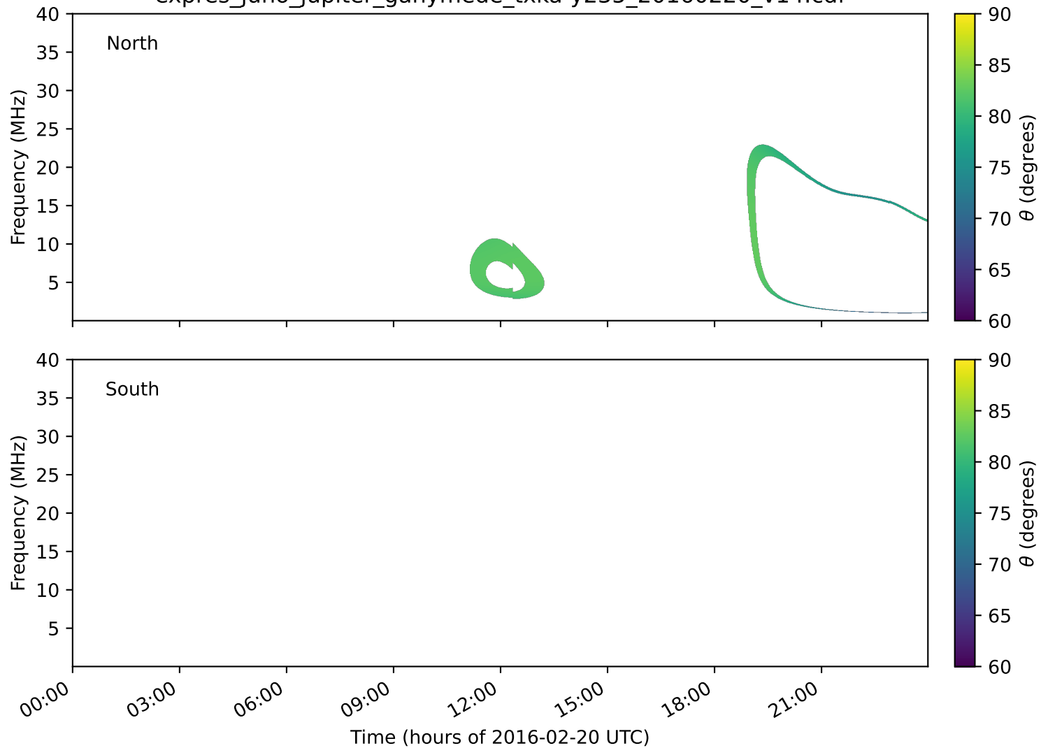
expres_juno_jupiter_ganymede_txka-y235_20160220_v14.cdf
