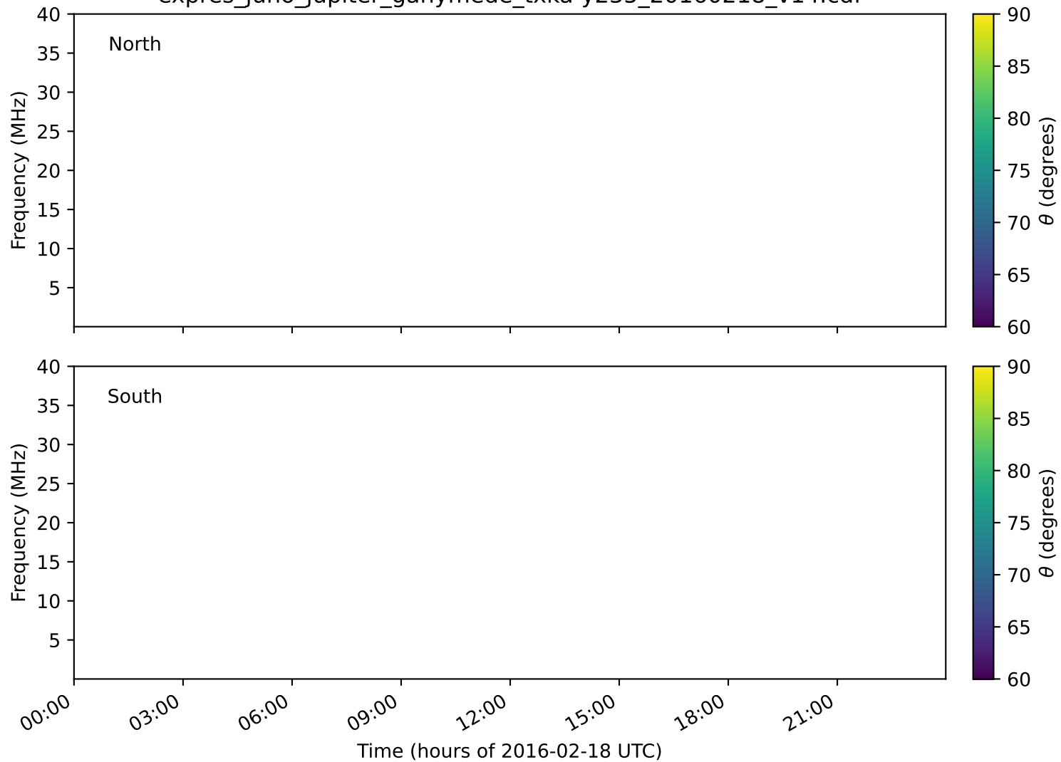
expres_juno_jupiter_ganymede_txka-y235_20160218_v14.cdf
