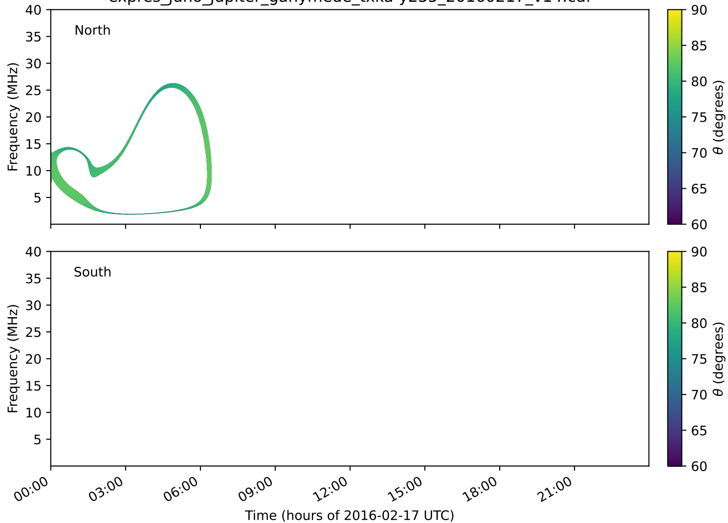
expres_juno_jupiter_ganymede_txka-y235_20160217_v14.cdf
