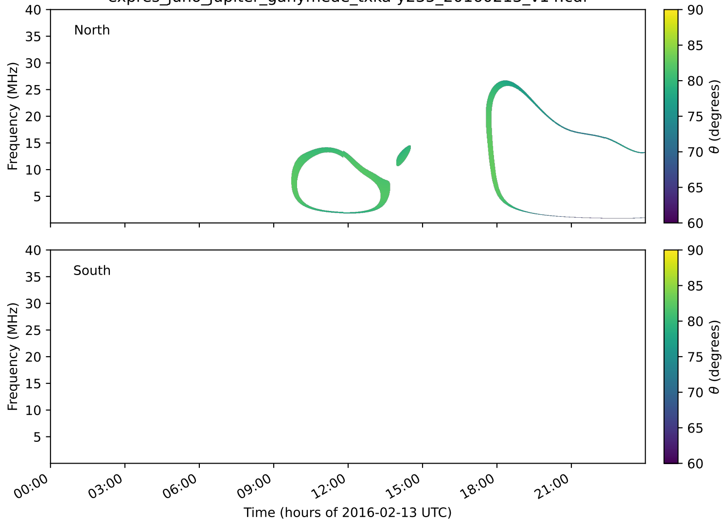
expres_juno_jupiter_ganymede_txka-y235_20160213_v14.cdf
