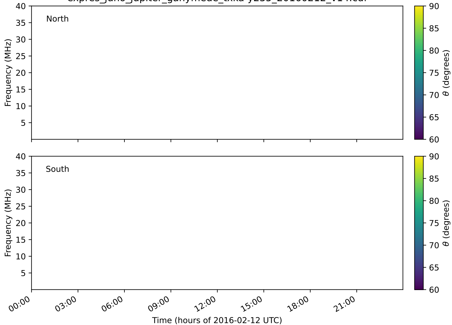
expres_juno_jupiter_ganymede_txka-y235_20160212_v14.cdf
