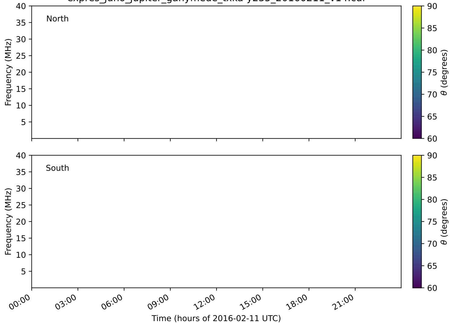
expres_juno_jupiter_ganymede_txka-y235_20160211_v14.cdf
