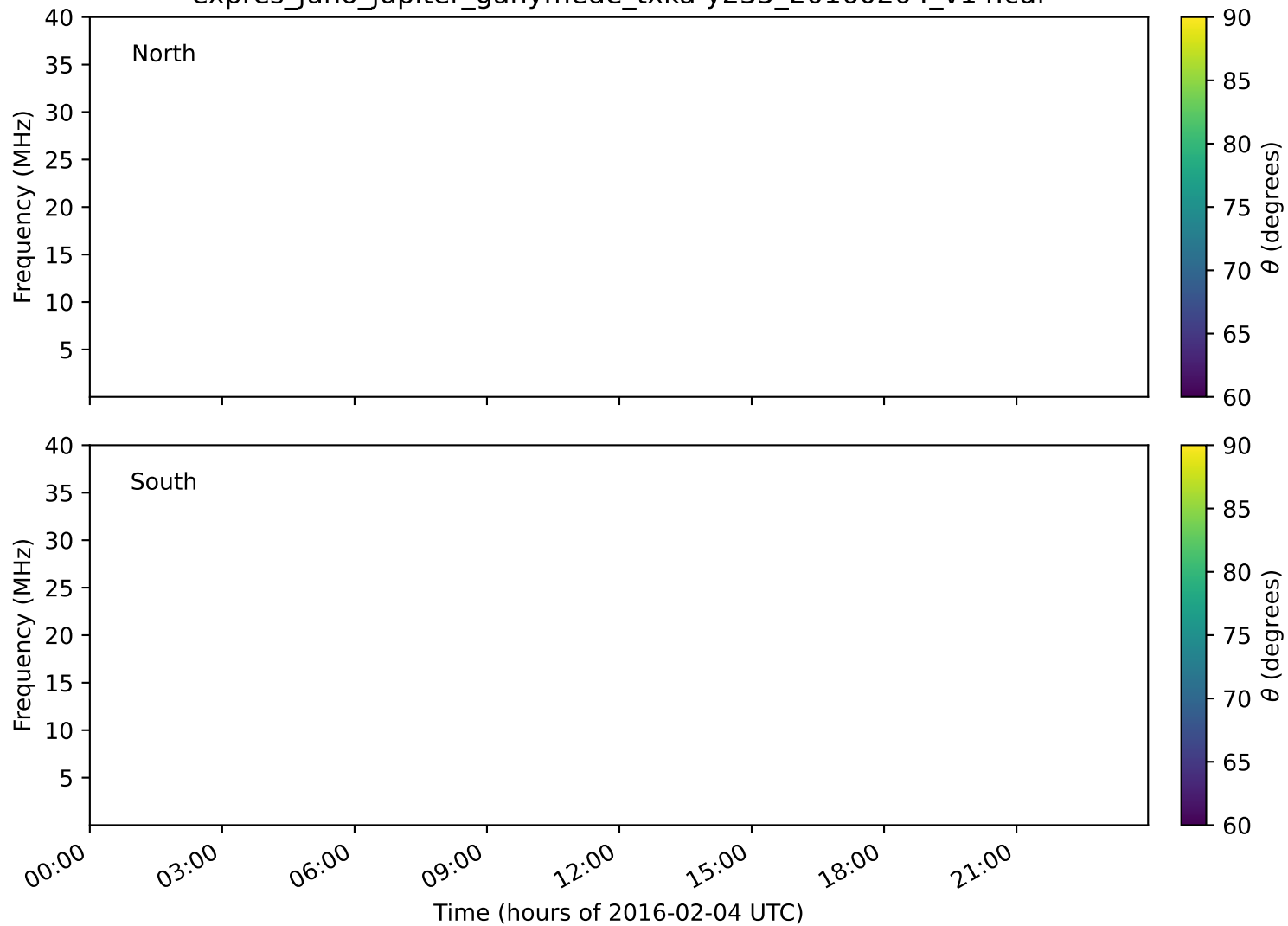
expres_juno_jupiter_ganymede_txka-y235_20160204_v14.cdf
