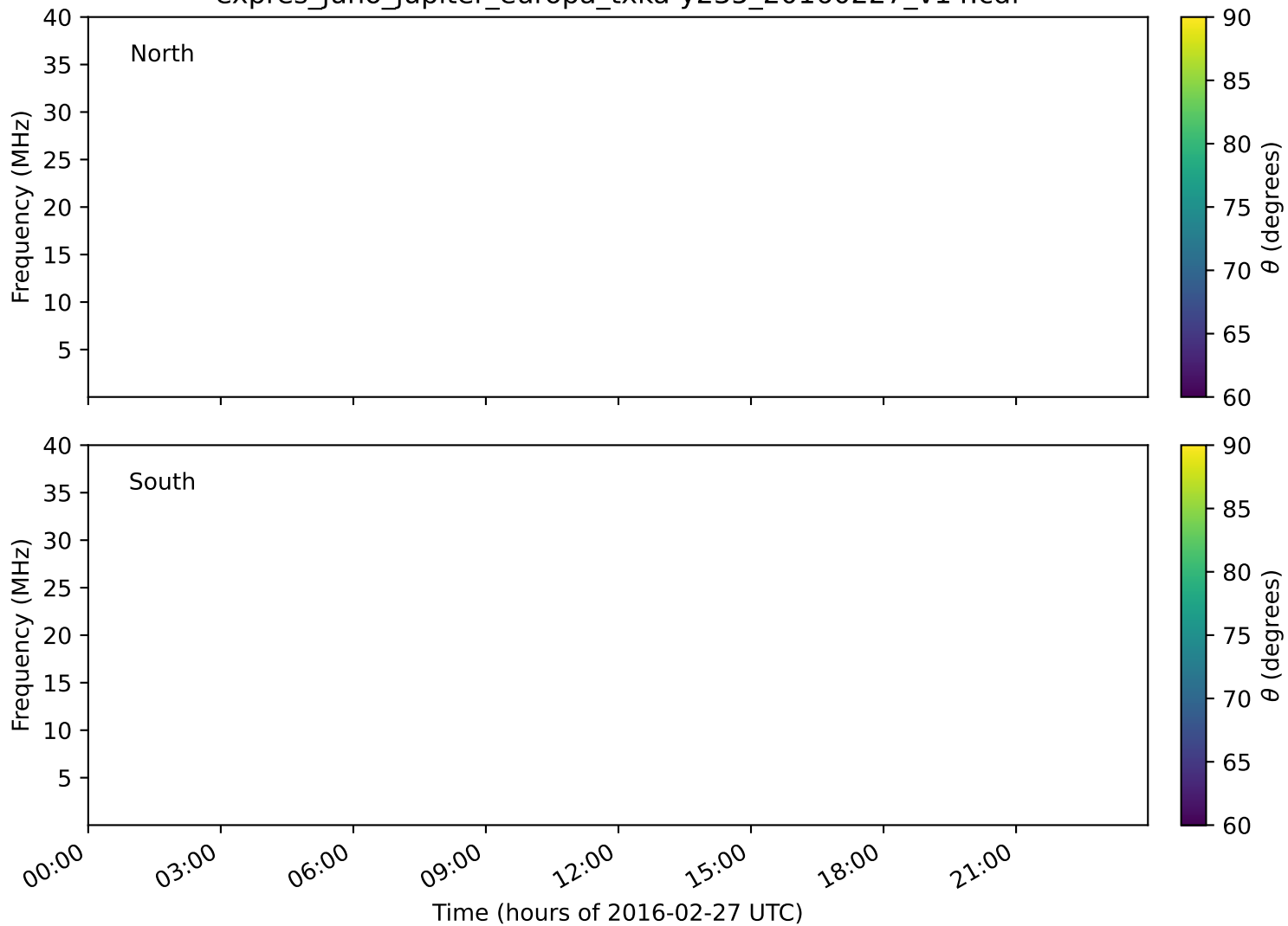
expres_juno_jupiter_europa_txka-y235_20160227_v14.cdf
