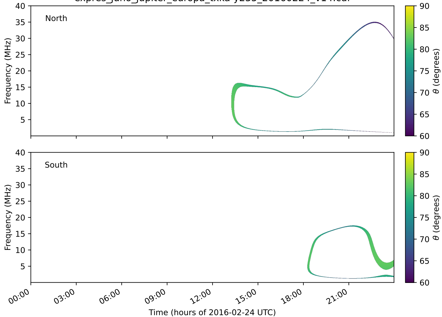
expres_juno_jupiter_europa_txka-y235_20160224_v14.cdf
