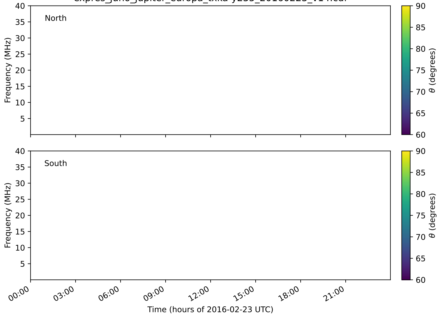
expres_juno_jupiter_europa_txka-y235_20160223_v14.cdf
