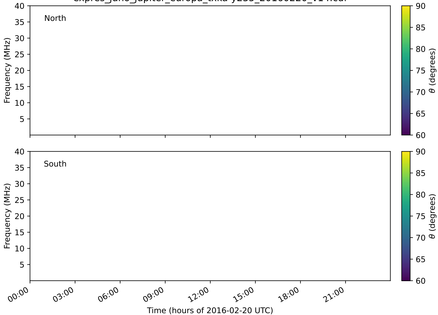
expres_juno_jupiter_europa_txka-y235_20160220_v14.cdf
