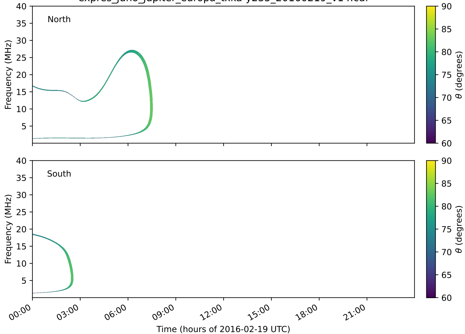
expres_juno_jupiter_europa_txka-y235_20160219_v14.cdf
