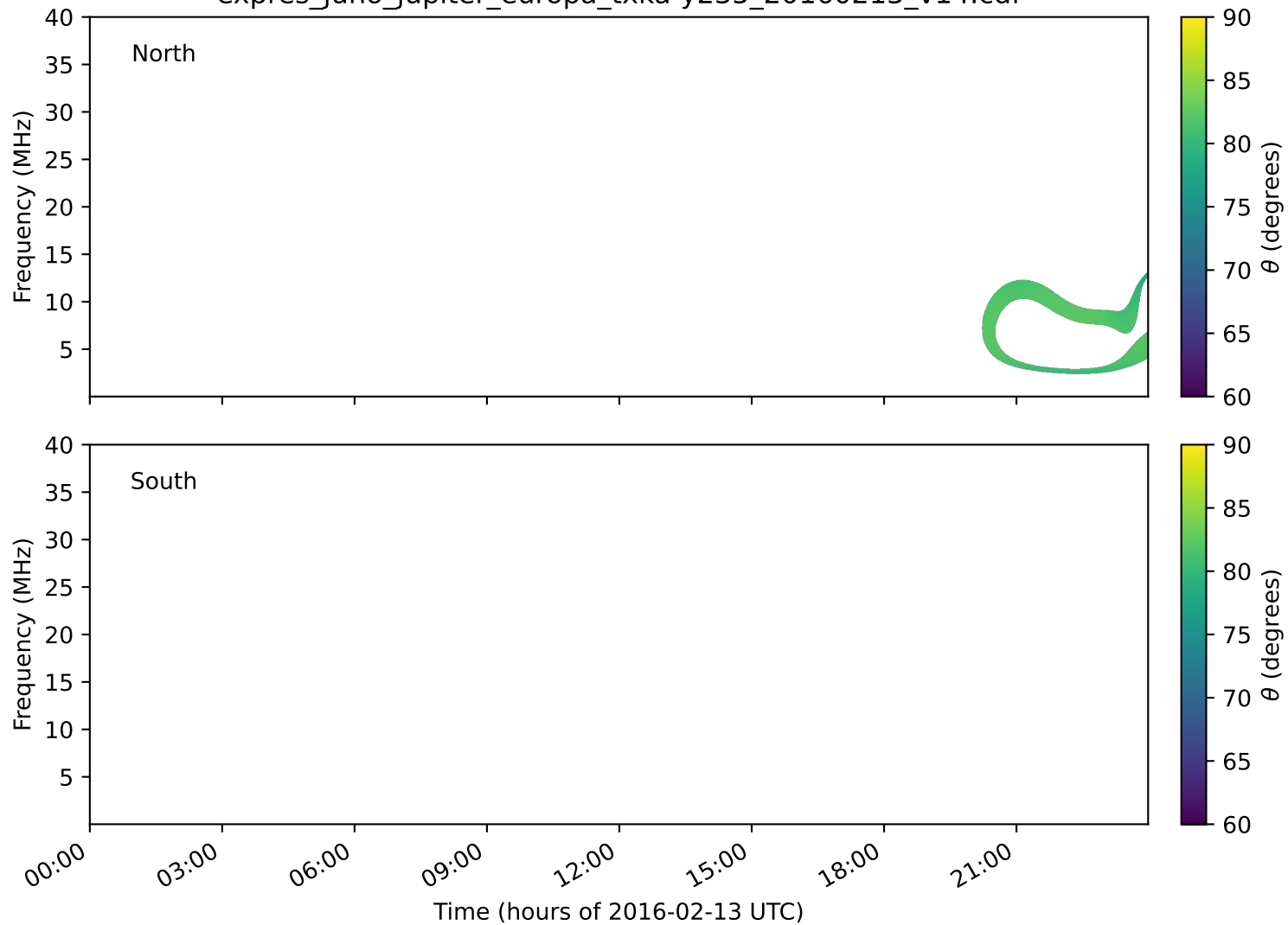
expres_juno_jupiter_europa_txka-y235_20160213_v14.cdf
