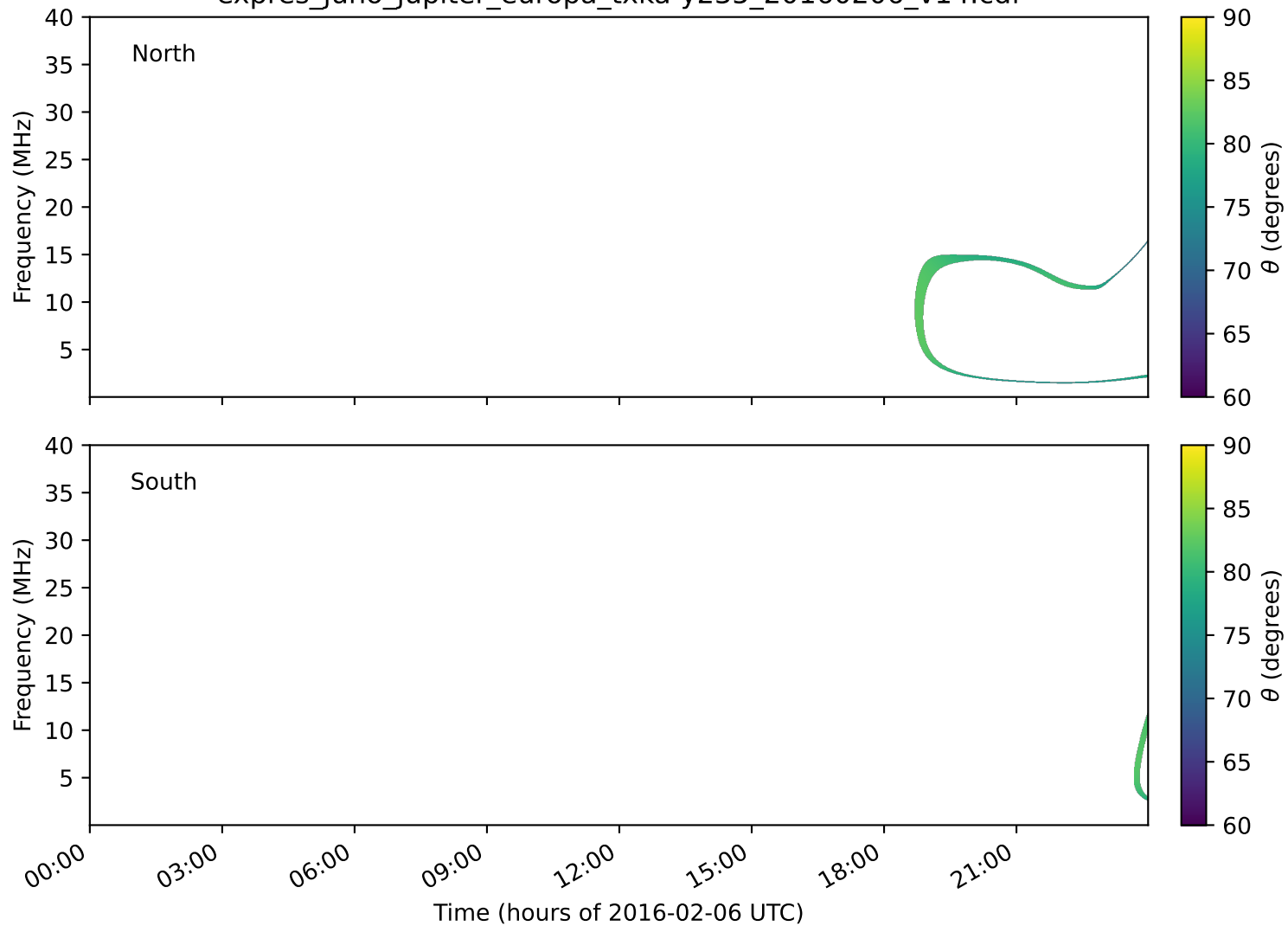
expres_juno_jupiter_europa_txka-y235_20160206_v14.cdf
