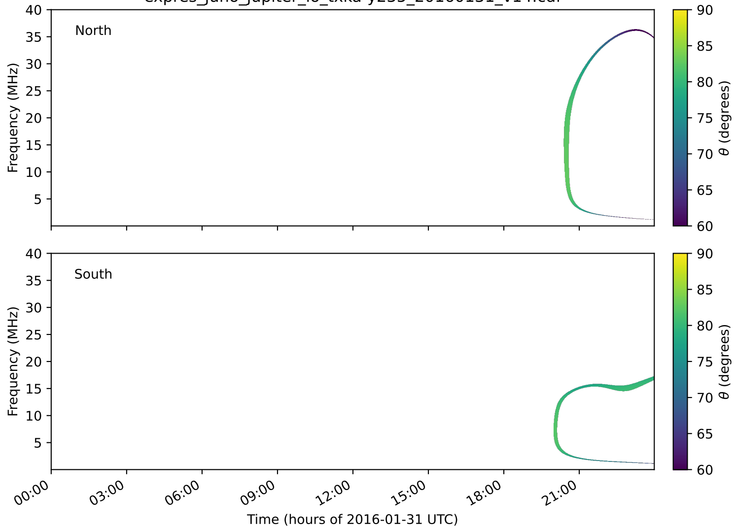
expres_juno_jupiter_io_txka-y235_20160131_v14.cdf
