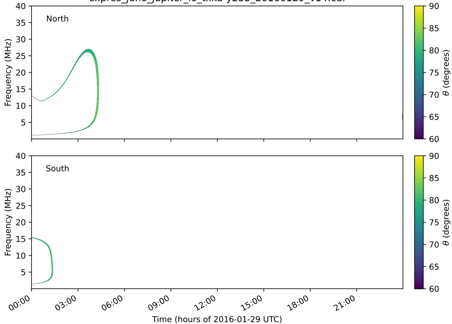
expres_juno_jupiter_io_txka-y235_20160129_v14.cdf
