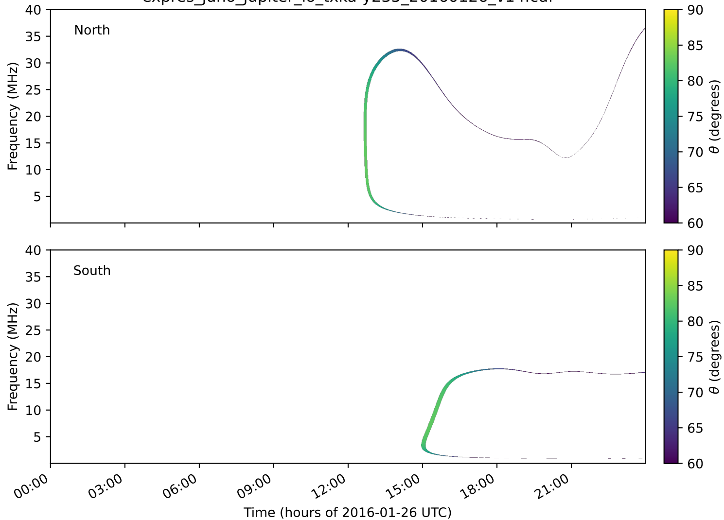
expres_juno_jupiter_io_txka-y235_20160126_v14.cdf
