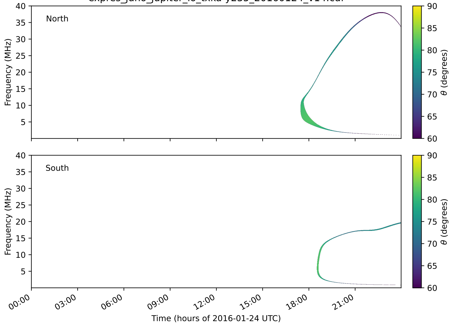
expres_juno_jupiter_io_txka-y235_20160124_v14.cdf
