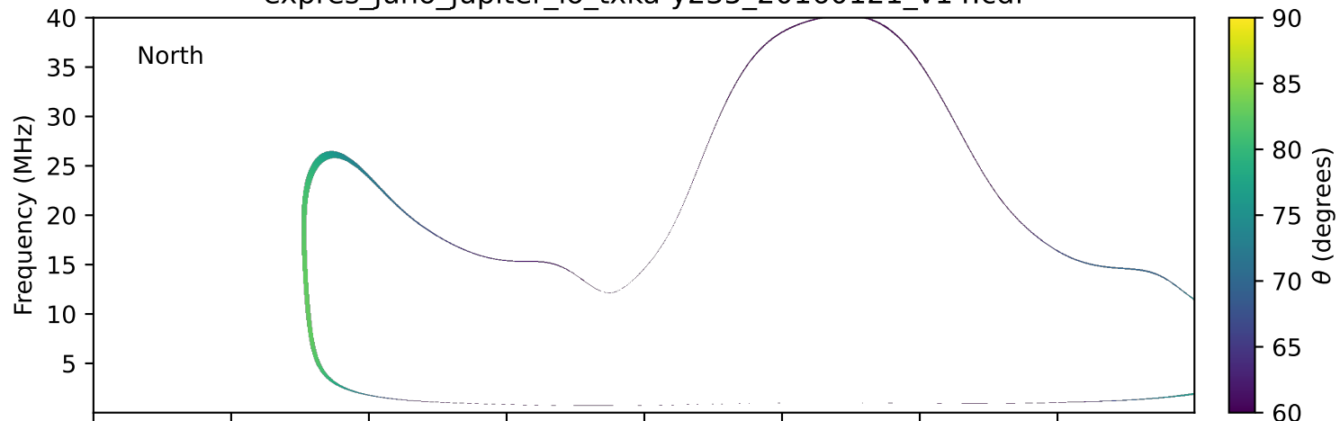
expres_juno_jupiter_io_txka-y235_20160121_v14.cdf
