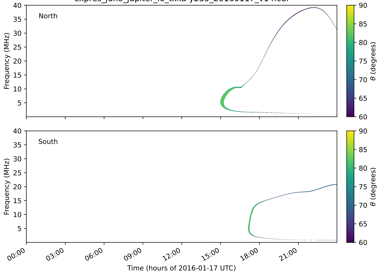
expres_juno_jupiter_io_txka-y235_20160117_v14.cdf
