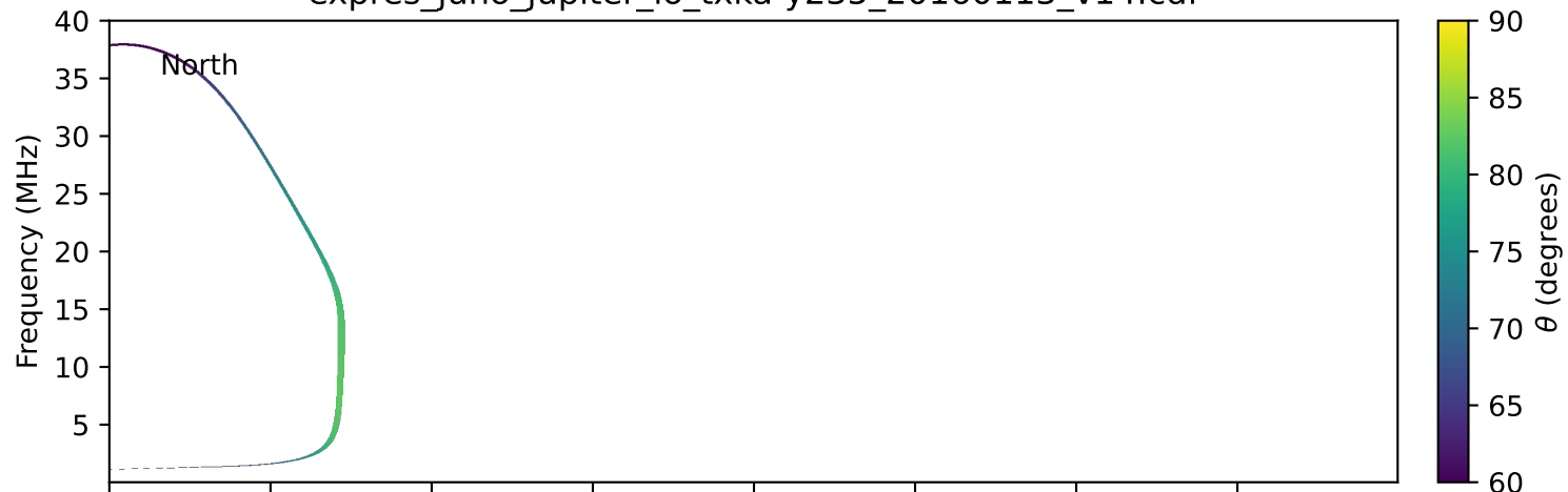
expres_juno_jupiter_io_txka-y235_20160113_v14.cdf
