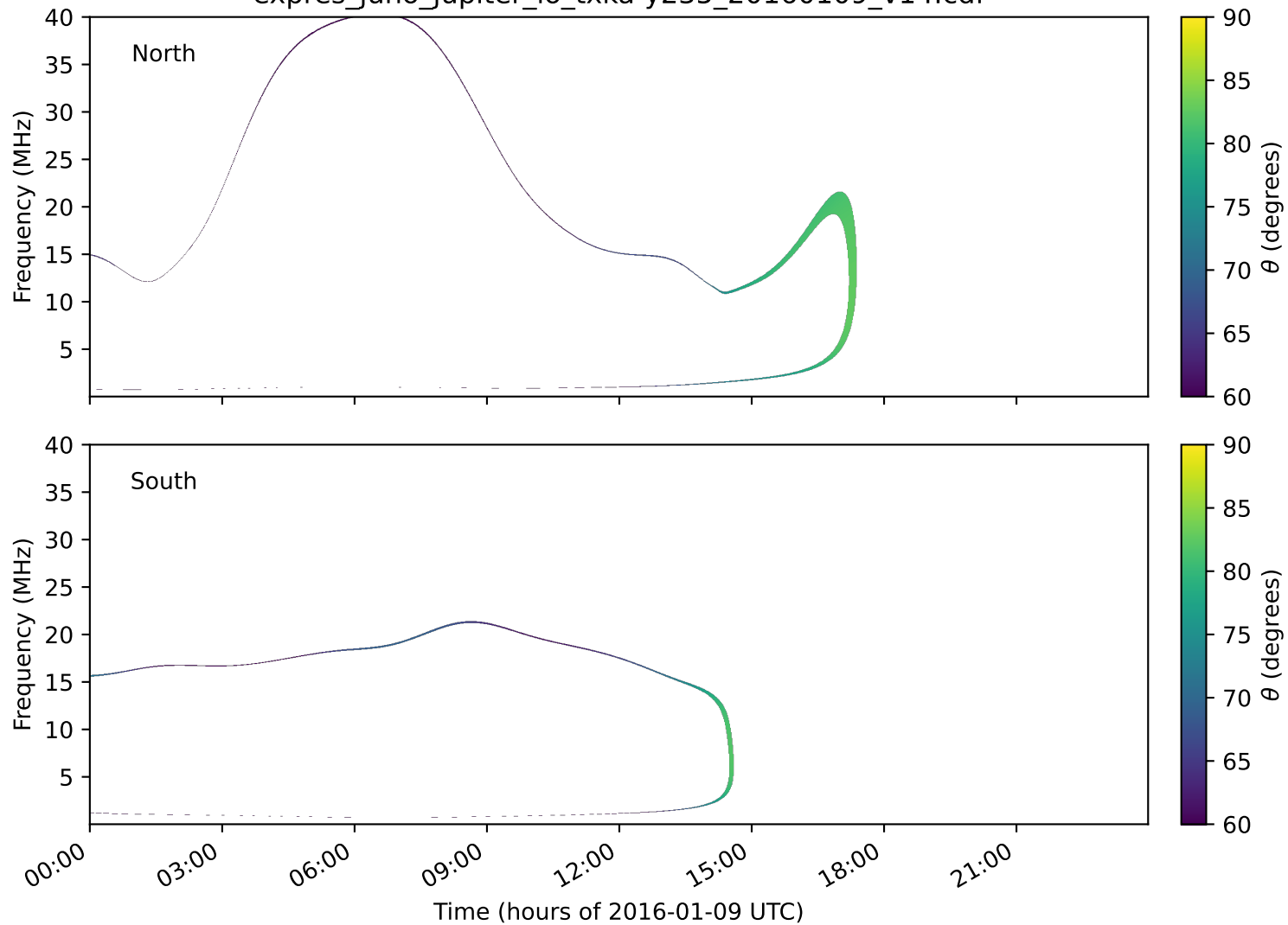
expres_juno_jupiter_io_txka-y235_20160109_v14.cdf
