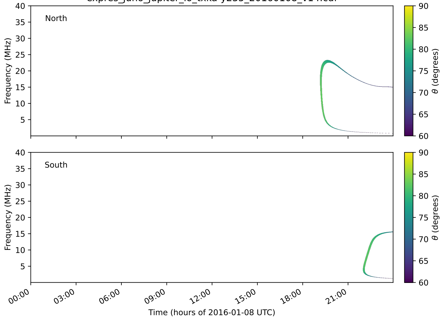
expres_juno_jupiter_io_txka-y235_20160108_v14.cdf
