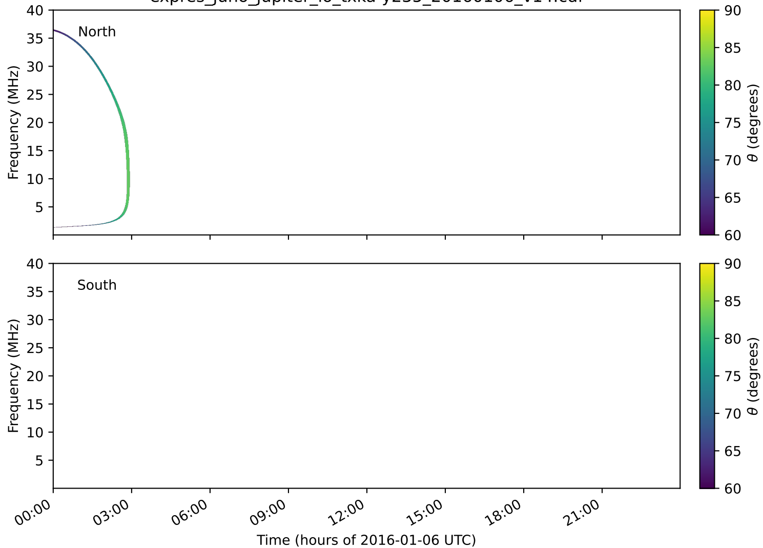
expres_juno_jupiter_io_txka-y235_20160106_v14.cdf
