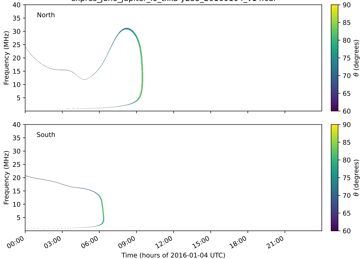
expres_juno_jupiter_io_txka-y235_20160104_v14.cdf
