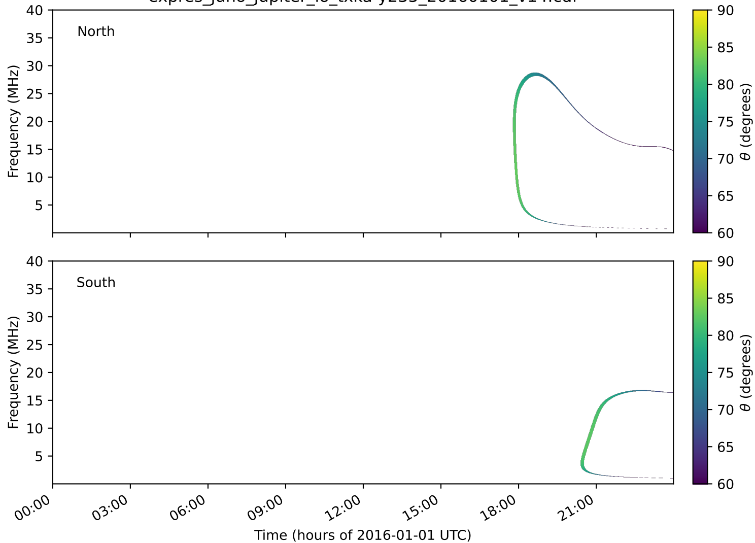
expres_juno_jupiter_io_txka-y235_20160101_v14.cdf
