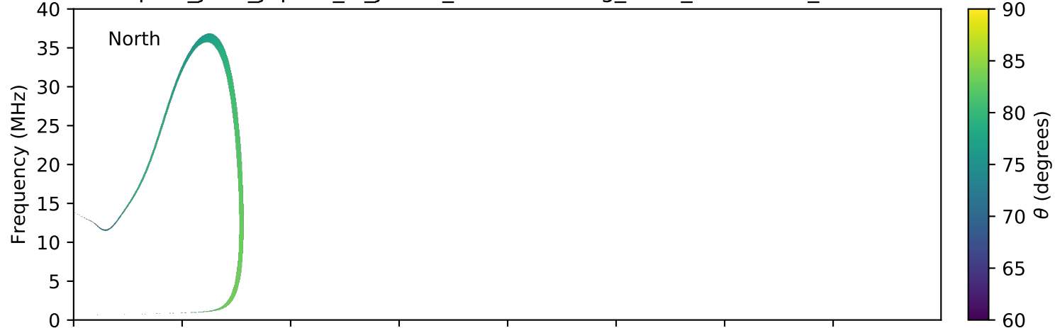
expres_juno_jupiter_io_jrm09_lossc-wid1deg_3kev_20160129_v01.cdf
