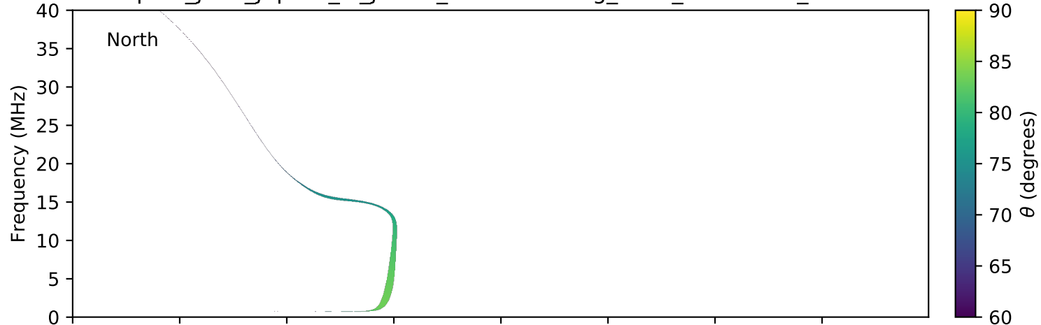
expres_juno_jupiter_io_jrm09_lossc-wid1deg_3kev_20160127_v01.cdf
