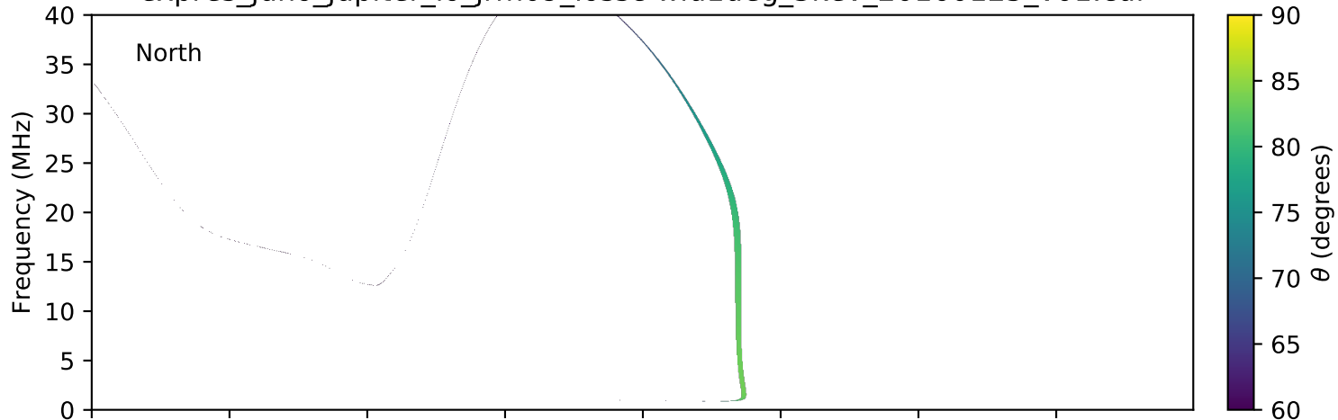
expres_juno_jupiter_io_jrm09_lossc-wid1deg_3kev_20160125_v01.cdf
