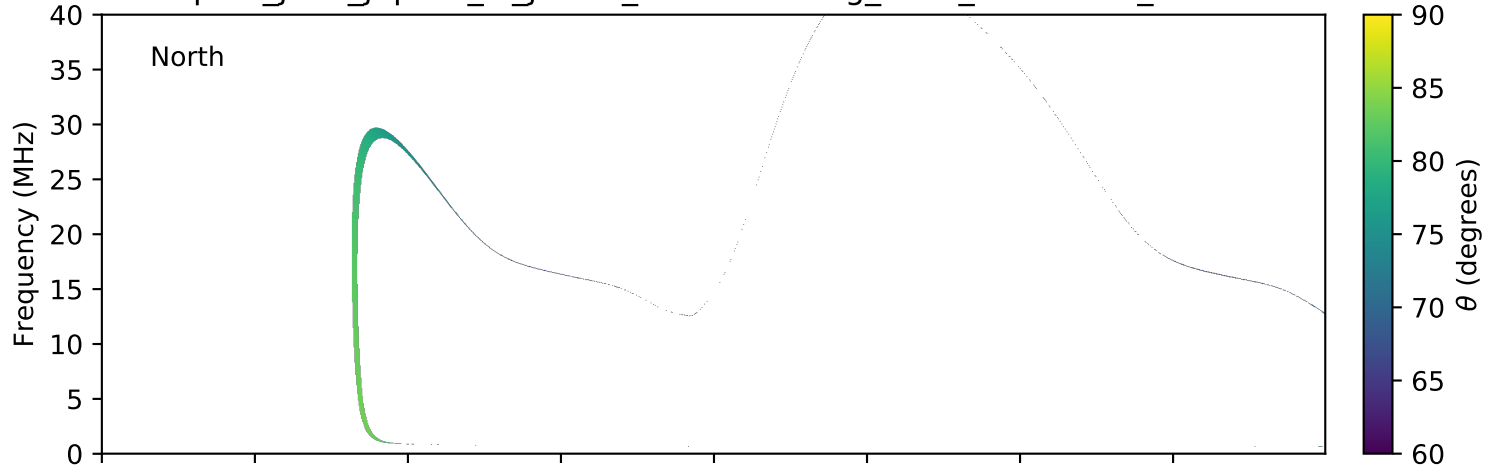
expres_juno_jupiter_io_jrm09_lossc-wid1deg_3kev_20160121_v01.cdf
