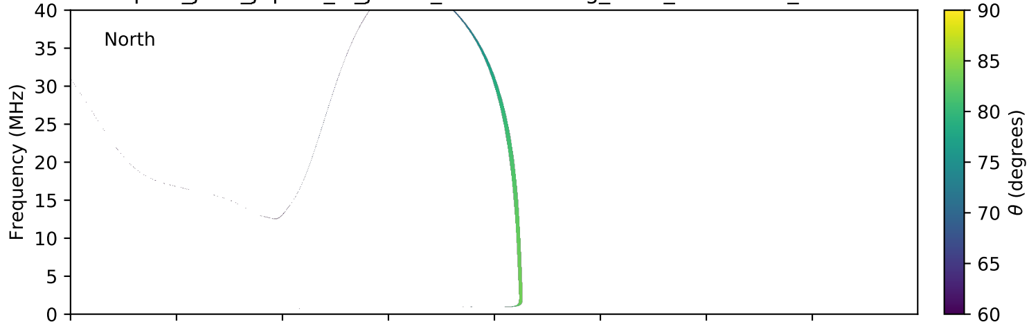
expres_juno_jupiter_io_jrm09_lossc-wid1deg_3kev_20160118_v01.cdf
