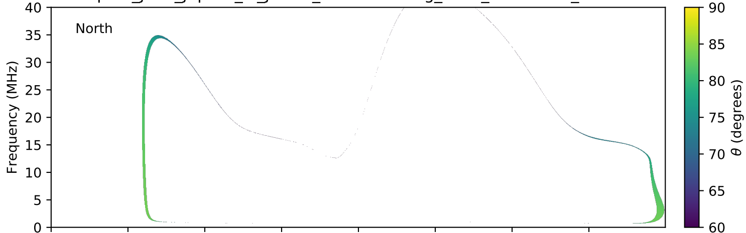
expres_juno_jupiter_io_jrm09_lossc-wid1deg_3kev_20160114_v01.cdf
