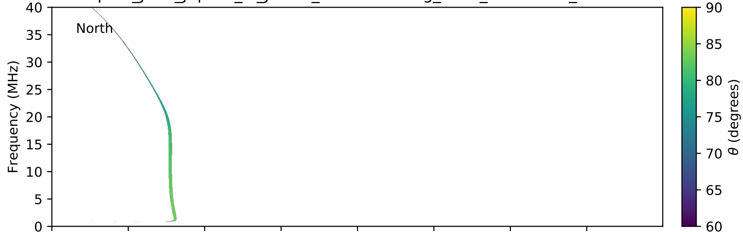
expres_juno_jupiter_io_jrm09_lossc-wid1deg_3kev_20160113_v01.cdf
