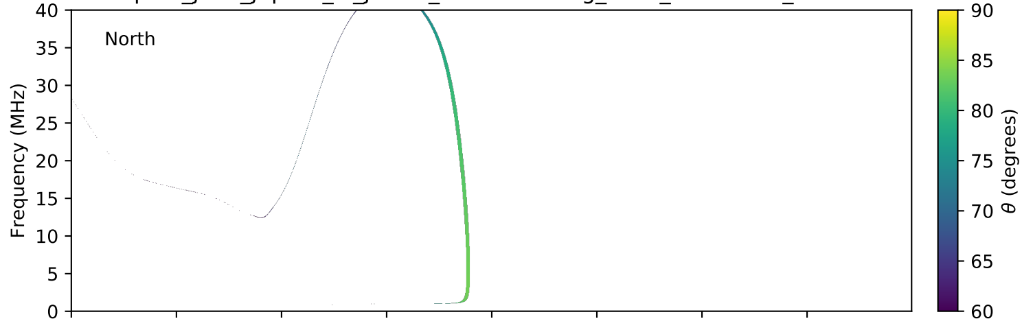
expres_juno_jupiter_io_jrm09_lossc-wid1deg_3kev_20160111_v01.cdf
