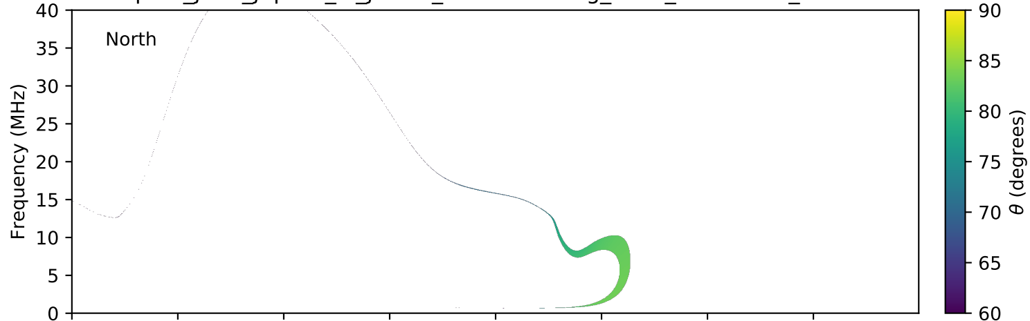
expres_juno_jupiter_io_jrm09_lossc-wid1deg_3kev_20160102_v01.cdf
