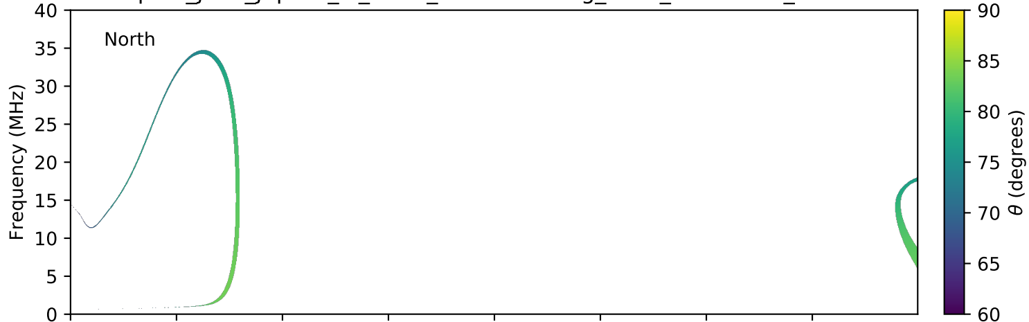
expres_juno_jupiter_io_isaac_lossc-wid1deg_3kev_20160129_v01.cdf
