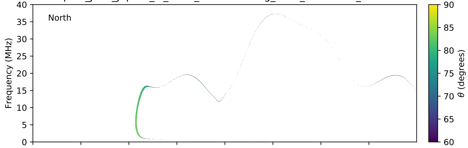
expres_juno_jupiter_io_isaac_lossc-wid1deg_3kev_20160128_v01.cdf
