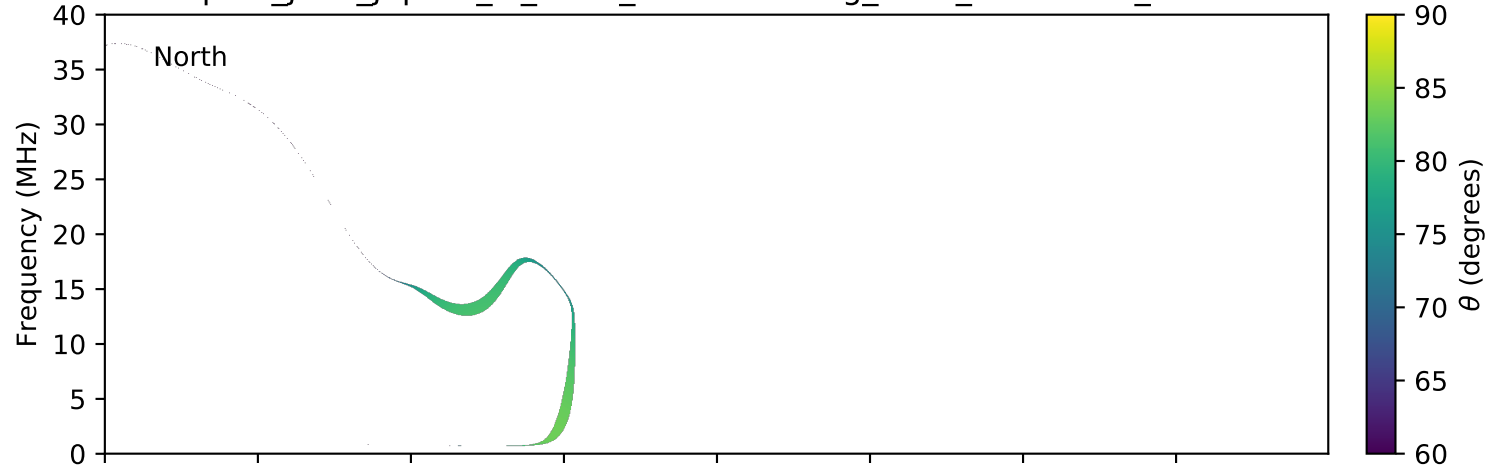
expres_juno_jupiter_io_isaac_lossc-wid1deg_3kev_20160127_v01.cdf
