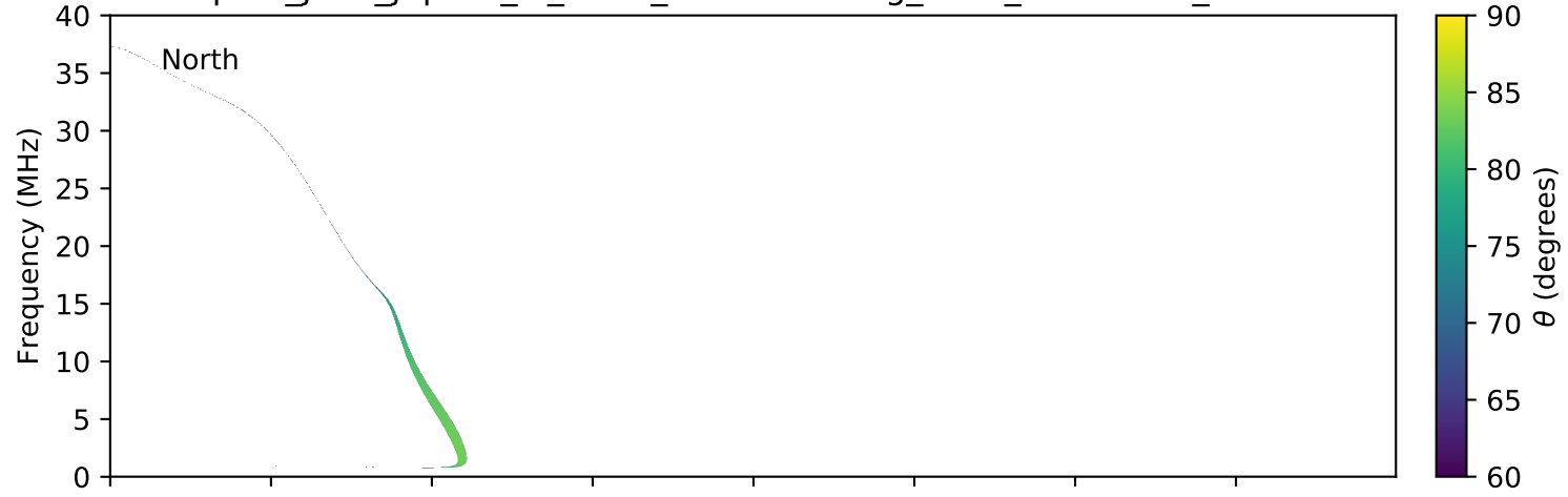
expres_juno_jupiter_io_isaac_lossc-wid1deg_3kev_20160120_v01.cdf
