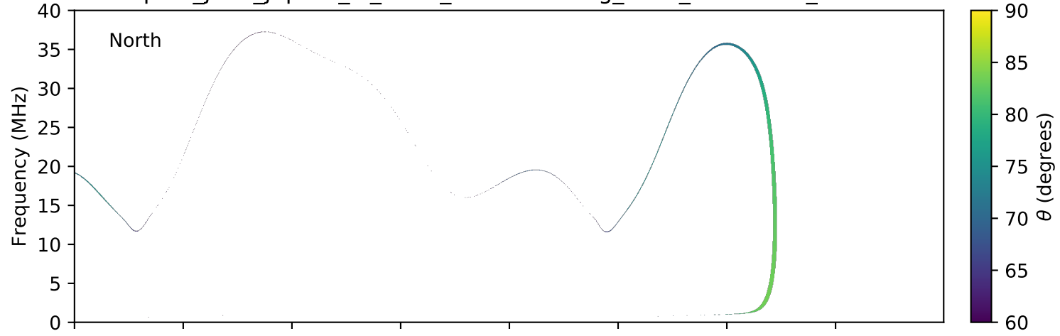
expres_juno_jupiter_io_isaac_lossc-wid1deg_3kev_20160116_v01.cdf
