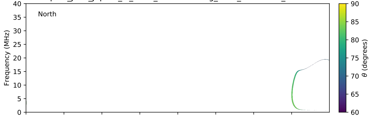
expres_juno_jupiter_io_isaac_lossc-wid1deg_3kev_20160115_v01.cdf
