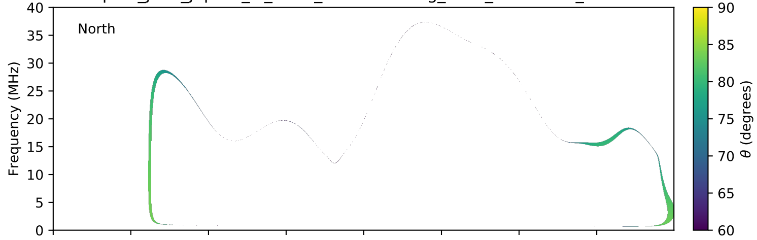
expres_juno_jupiter_io_isaac_lossc-wid1deg_3kev_20160114_v01.cdf
