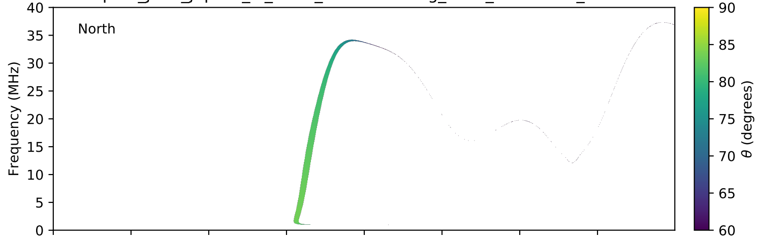
expres_juno_jupiter_io_isaac_lossc-wid1deg_3kev_20160112_v01.cdf
