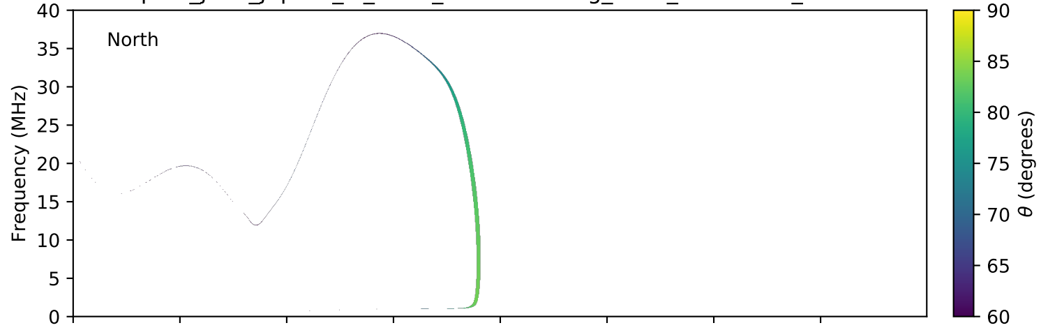
expres_juno_jupiter_io_isaac_lossc-wid1deg_3kev_20160111_v01.cdf
