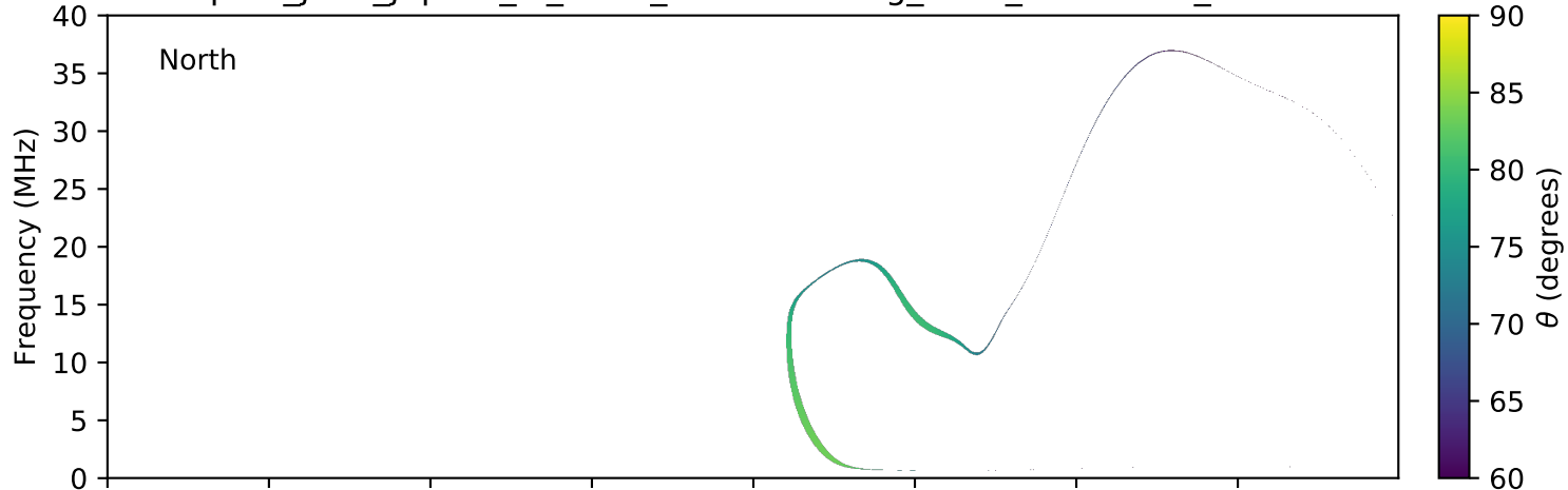
expres_juno_jupiter_io_isaac_lossc-wid1deg_3kev_20160110_v01.cdf
