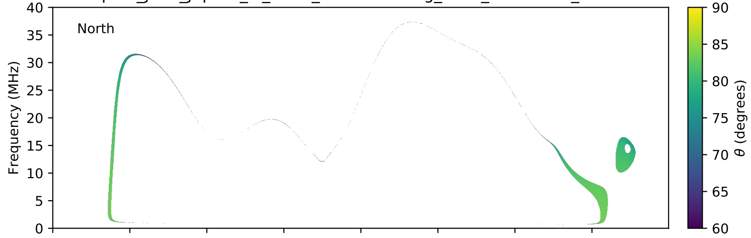
expres_juno_jupiter_io_isaac_lossc-wid1deg_3kev_20160107_v01.cdf
